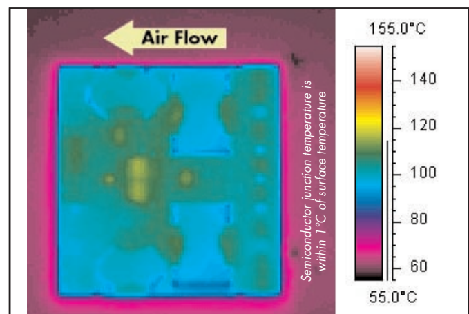
Figure 6: Thermal plot of converter at 40 amp load current with 55°C air flowing at the rate of 200 LFM. Air is flowing across the converter from output to input (nominal input voltage).
